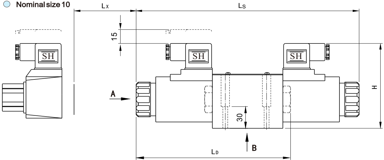
AC Plug-in Connection Type
