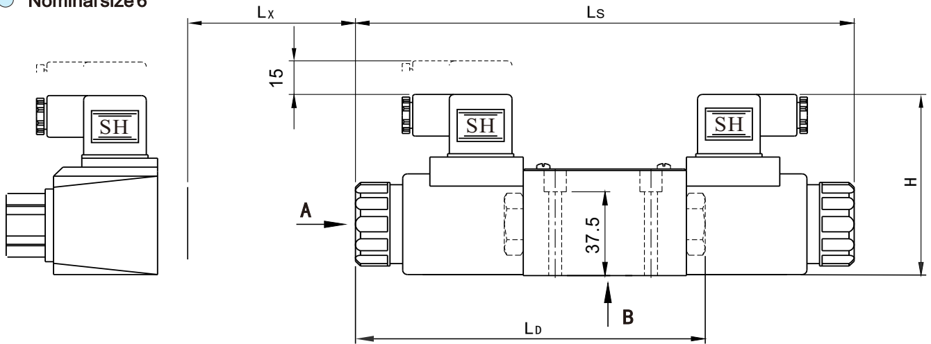
AC Plug-in Connection Type
